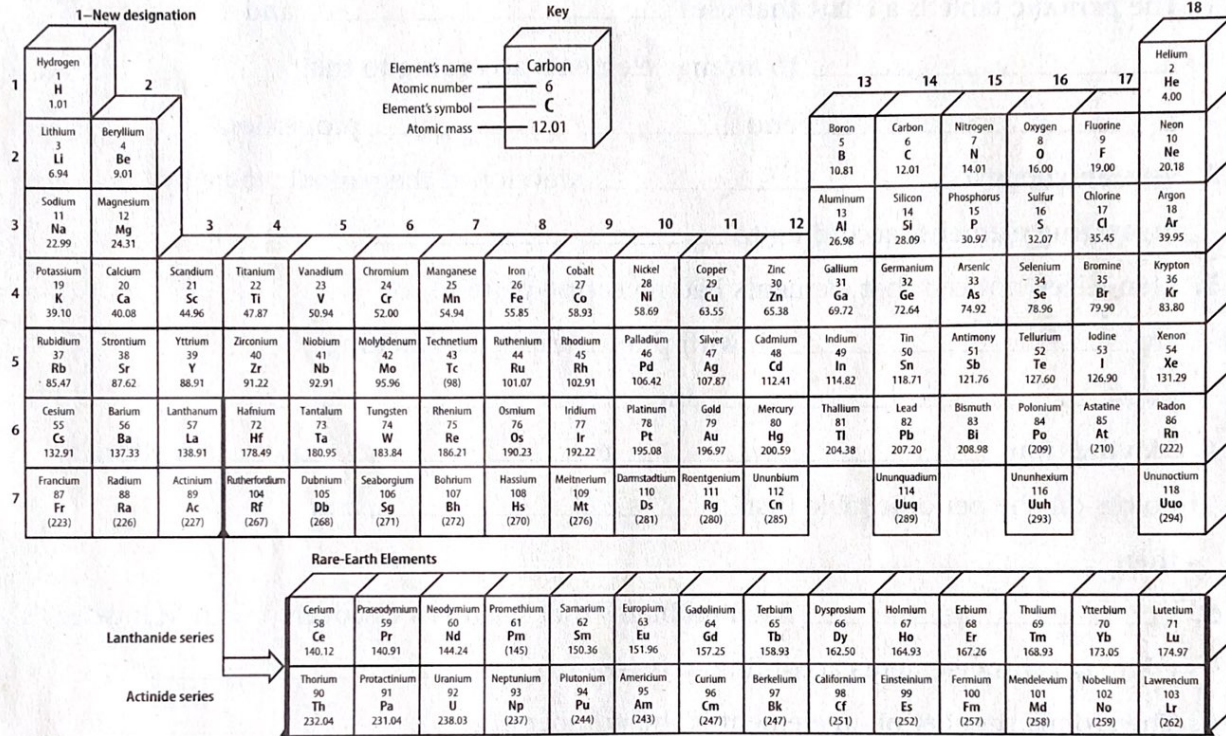
Periodic Table of the Elements
